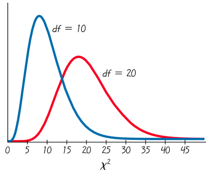
Figure 7-9 Chi-Square Distribution for df = 10 and df = 20
